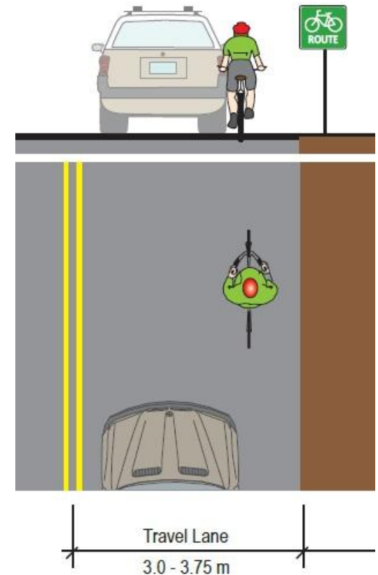
Shared space on a local road Elora, ON
