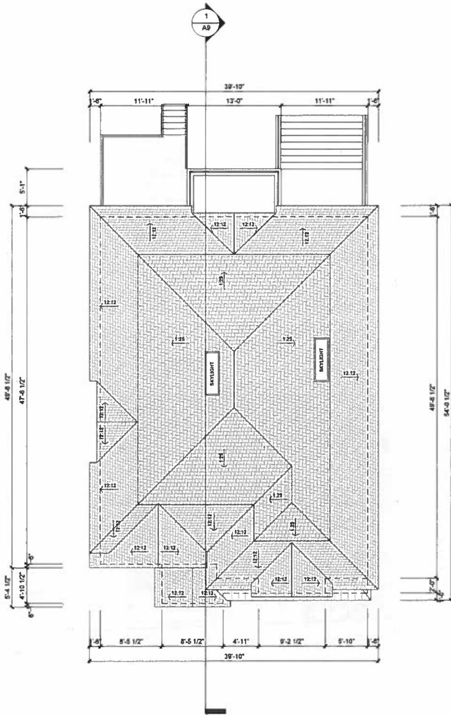
ROOF PLAN
