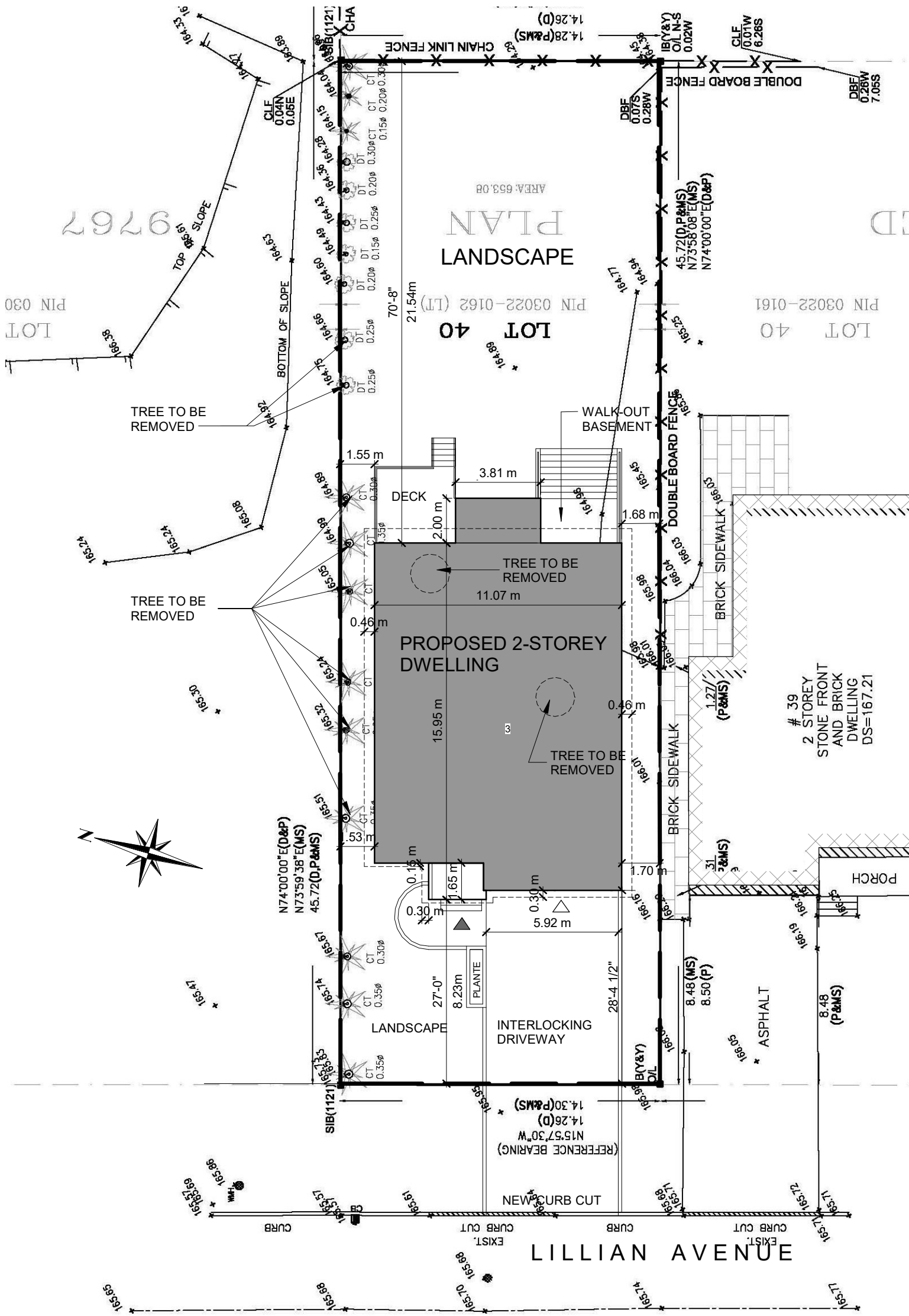
SITE PLAN
