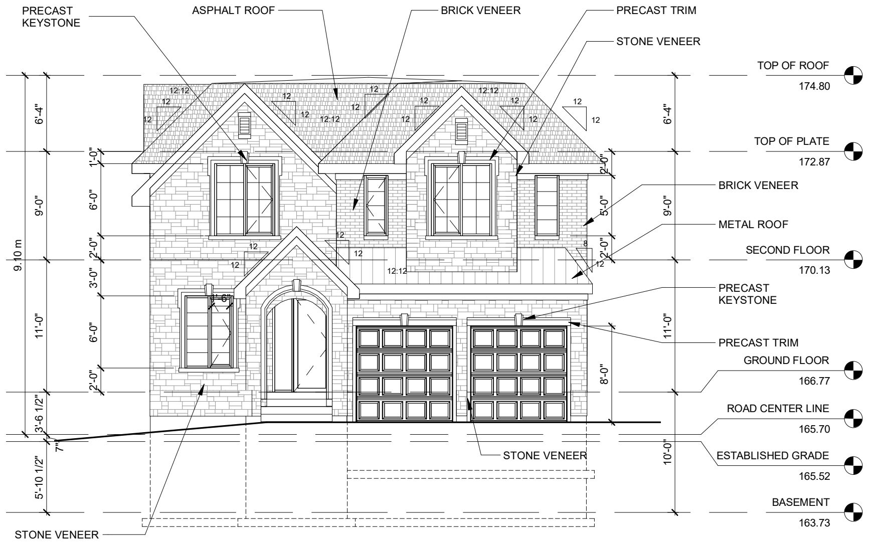
WEST ELEVATION
