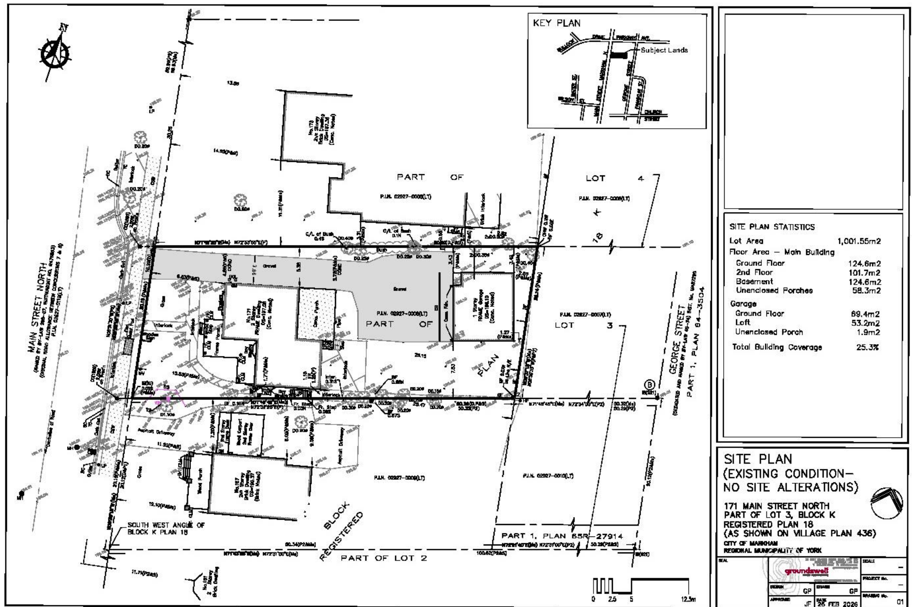
Figure 4: Site Plan
