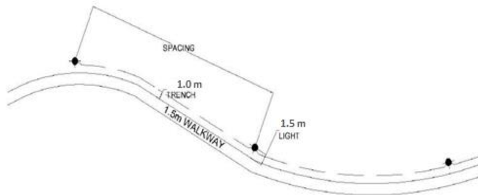
FIGURE 6: WALKWAY LIGHT INSTALLATION
